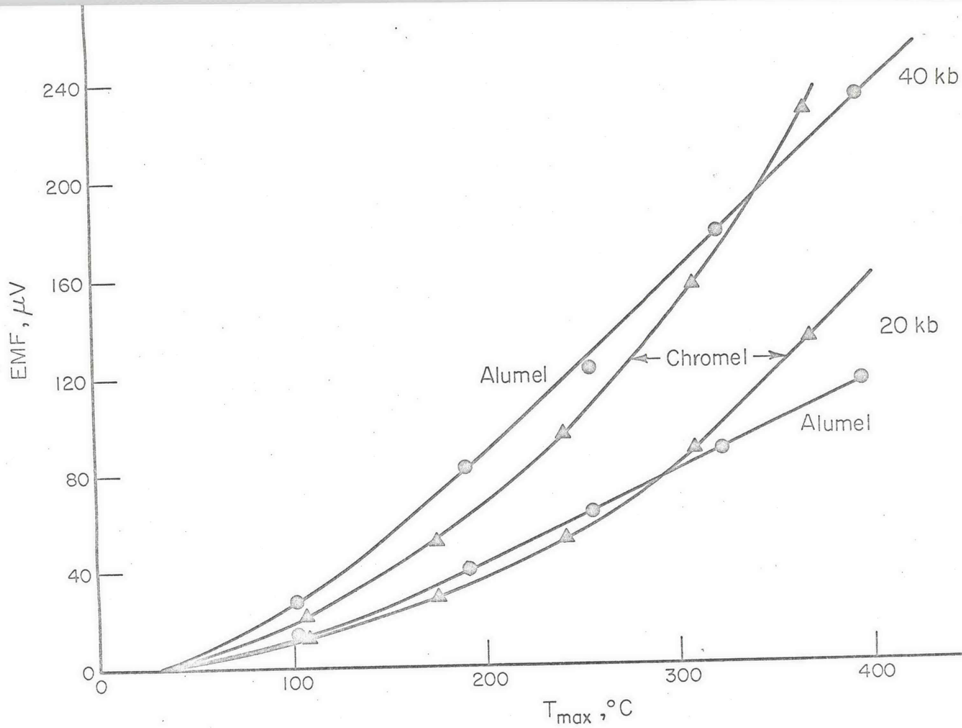
PRESSURE EMF VERSUS TEMPERATURE CHROMEL-ALUMEL Cold + ; hot -
